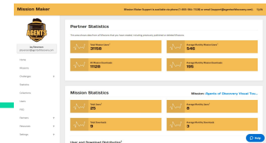
Statistics
